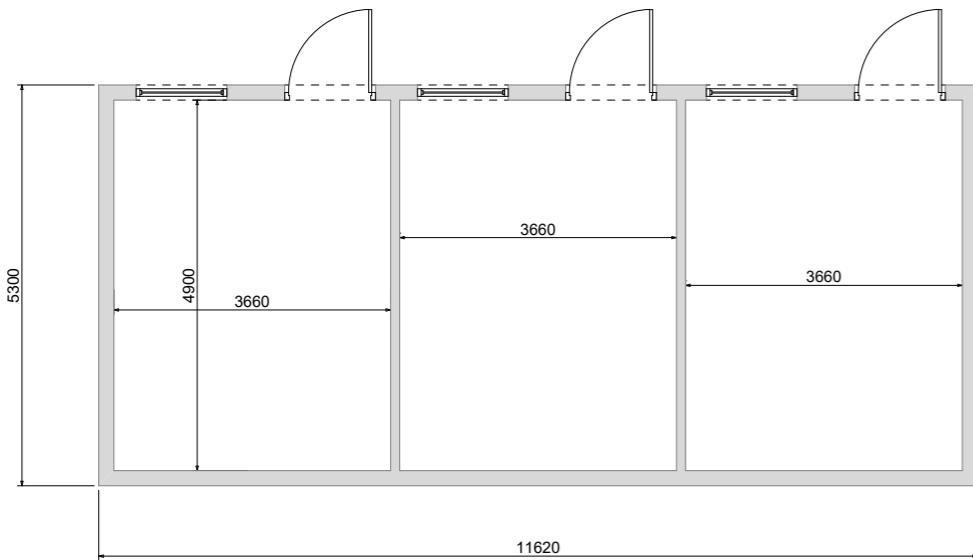
FLOOR PLAN
